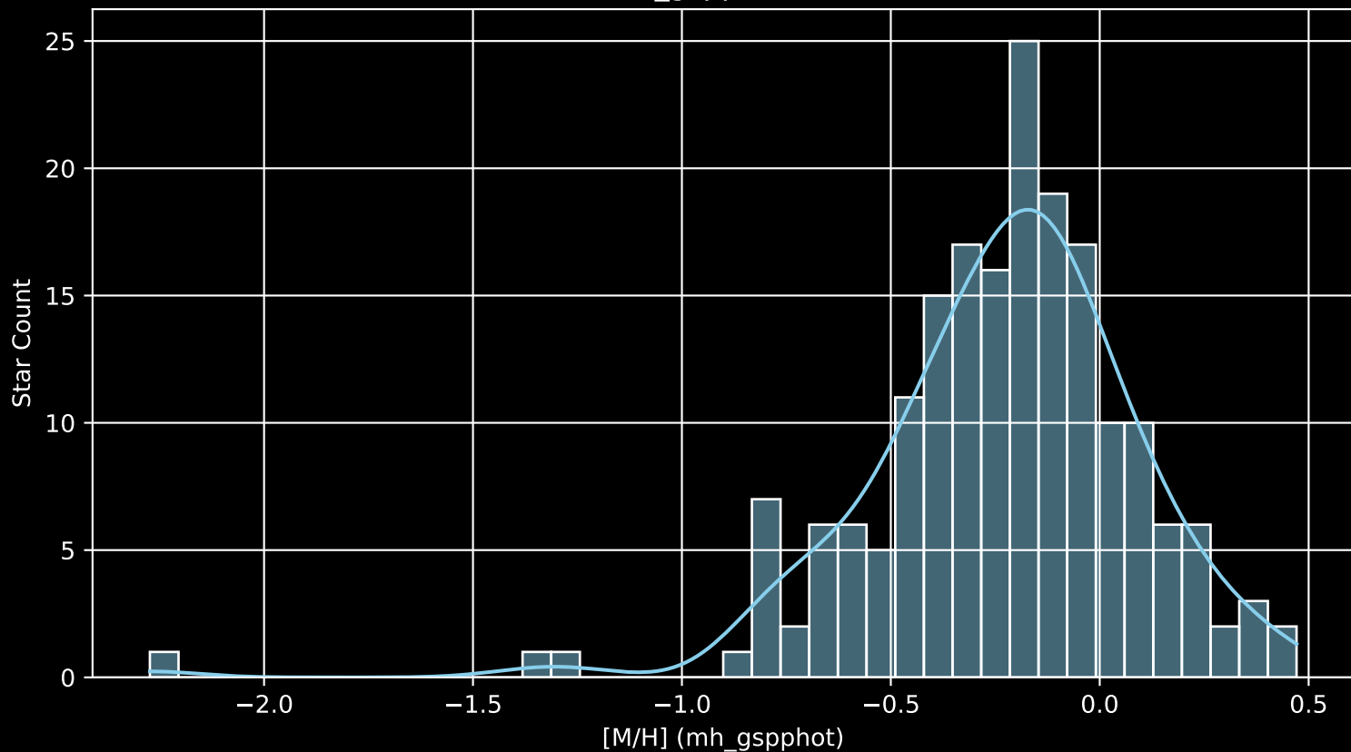
APOGEE DR17 Field: [094+61_MGA [M/H] (mh_gspphot) (n= 189)
