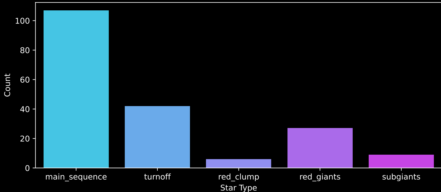
APOGEE DR17 Field: [094+61_MGA] Count plot of Star Type
