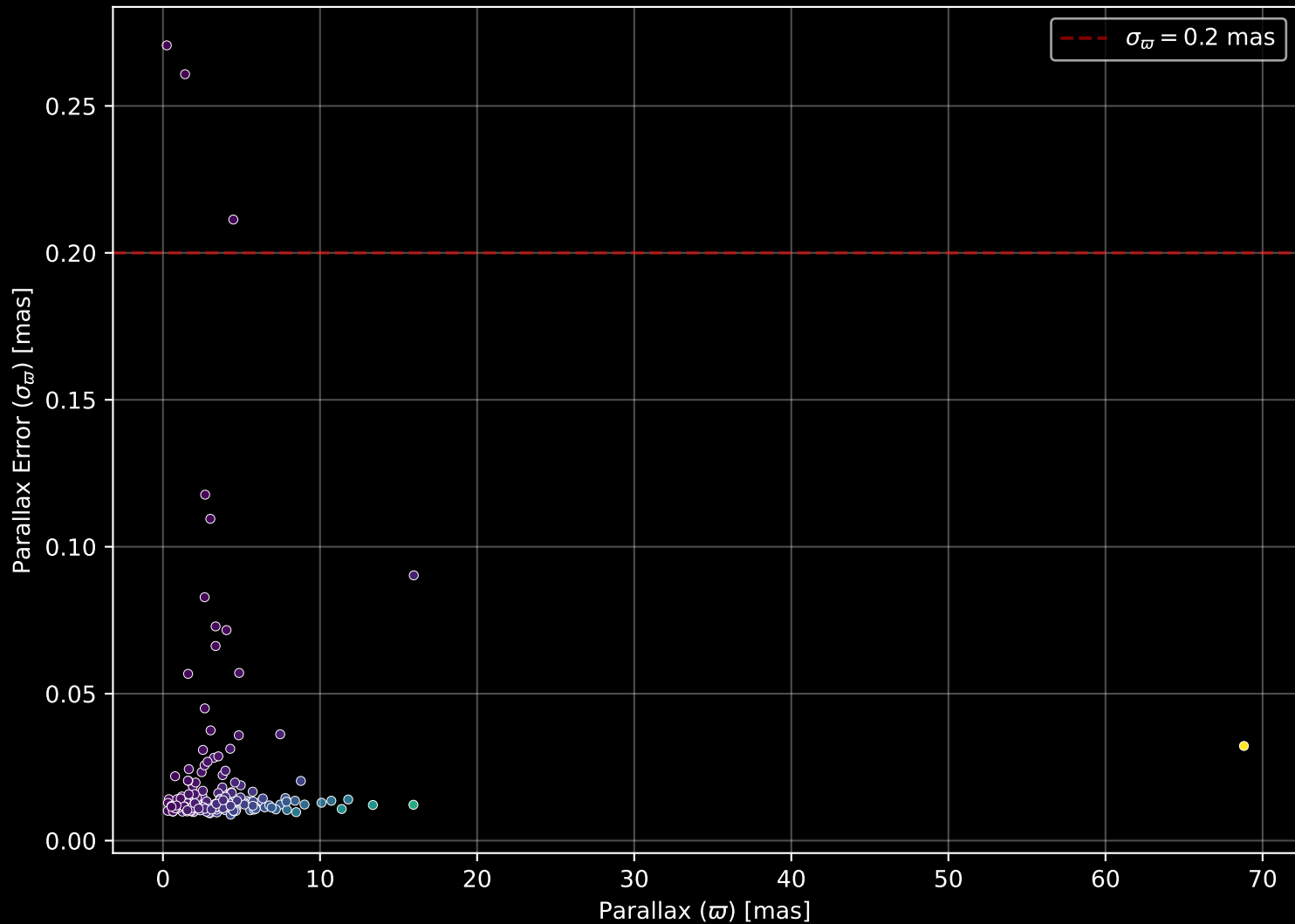
APOGEE DR17 Field: [094+61_MGA] Parallax Quality (n= 191)
