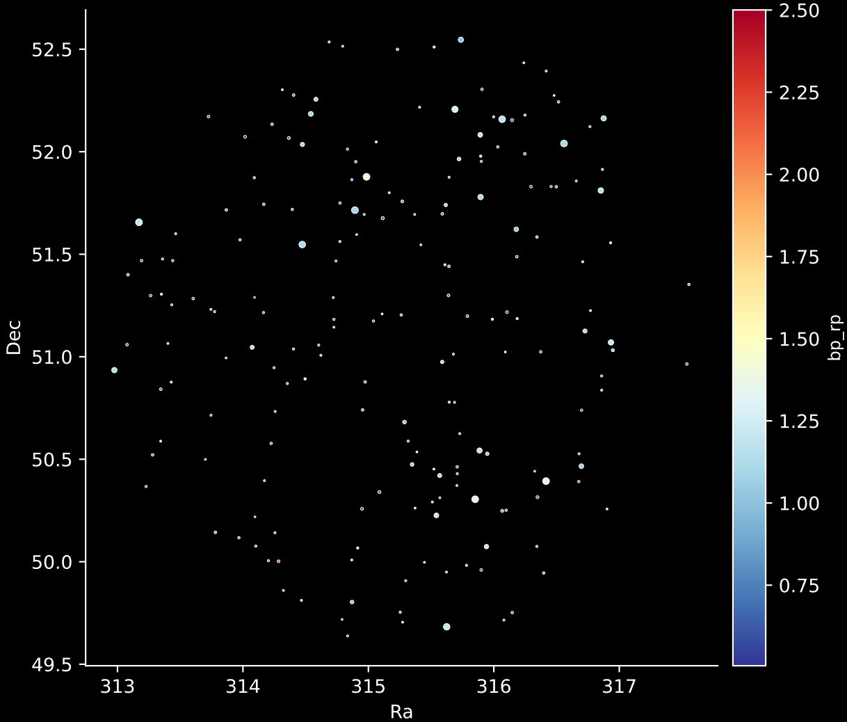
APOGEE DR17 Field: [094+61_MGA] Stars: 191
