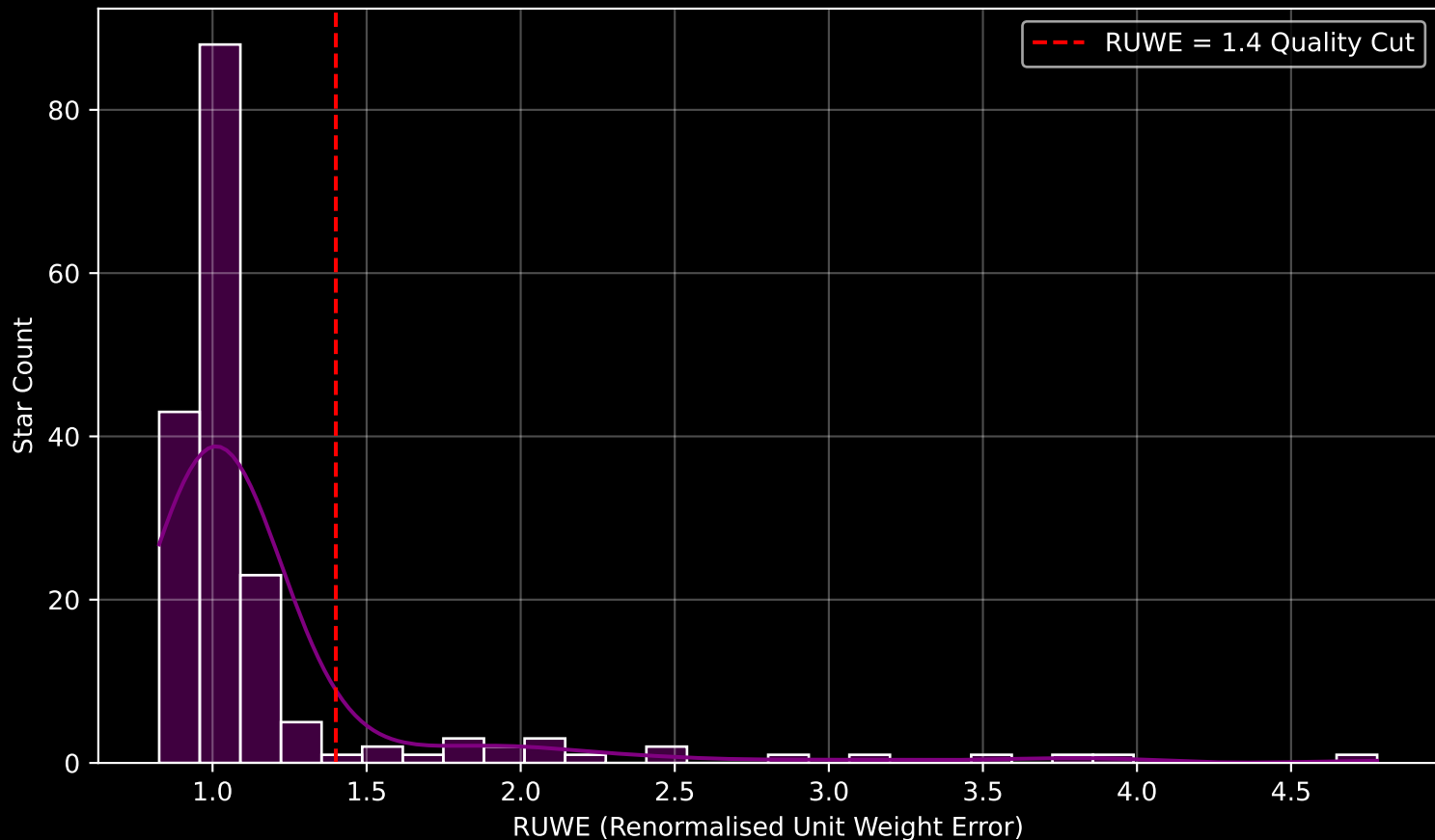
GAPOGEE DR17 Field [094+61_MGA] RUWE Distribution (n= 180)
