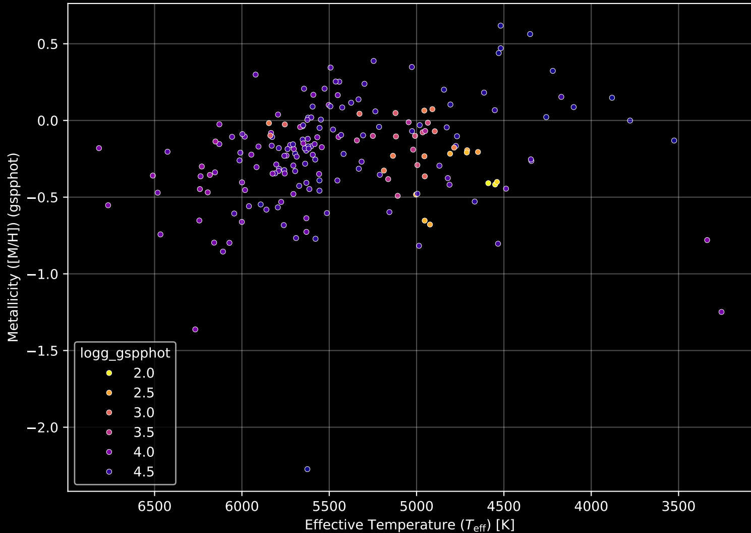
APOGEE DR17 Field: [094+61_MGA] Stellar Population Parameters (n= 191)
