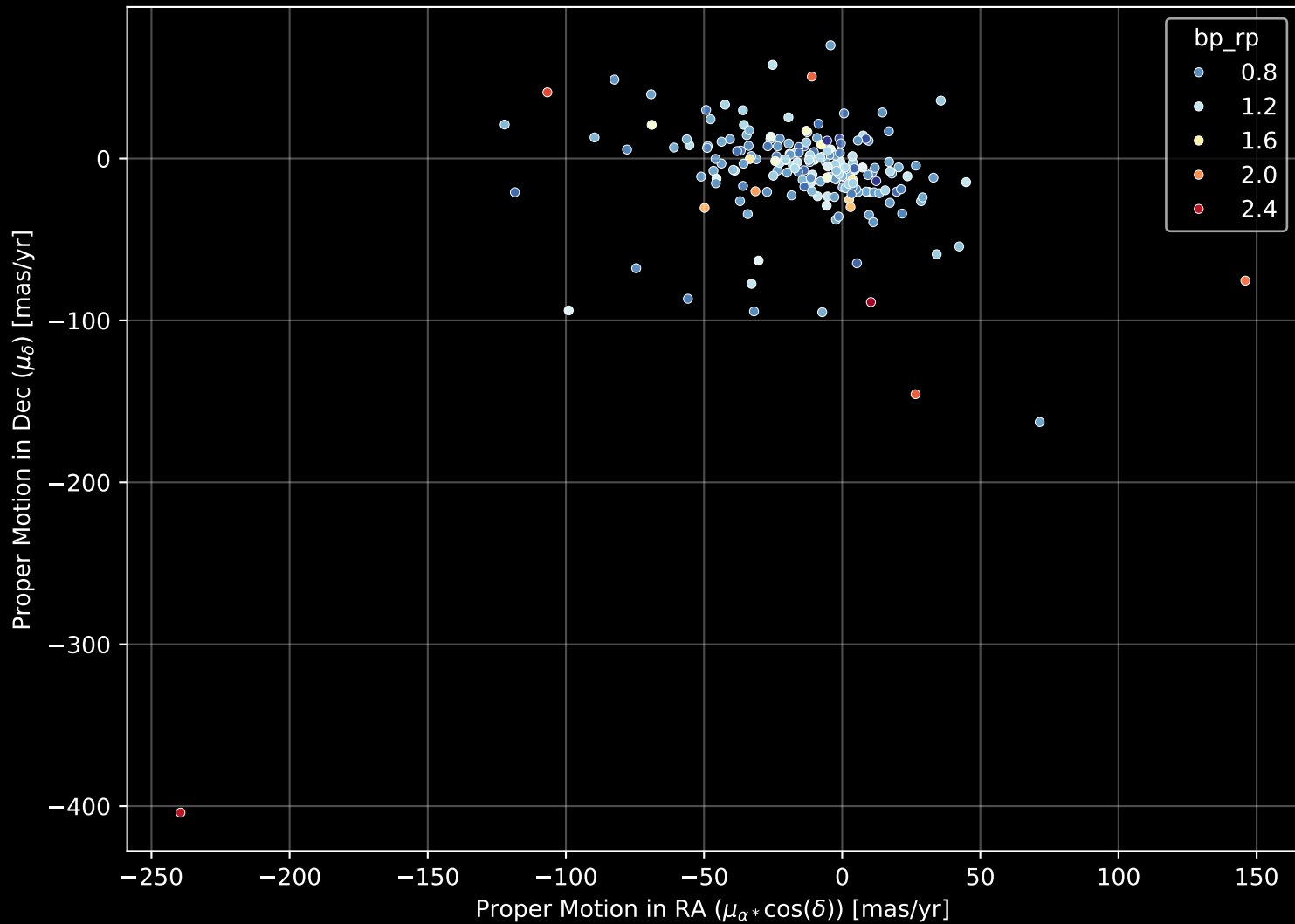
APOGEE DR17 Field: [094+61_MGA] Proper Motion Diagram (n= 191)
